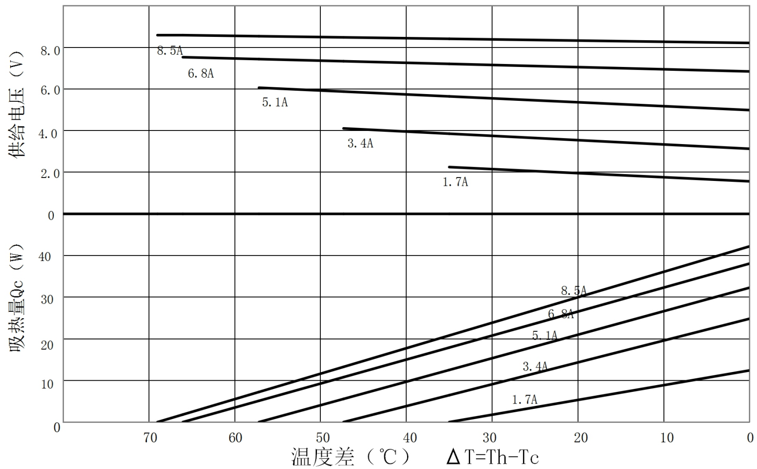
TEC1-B7108AC特性图 (Th=27°C)
