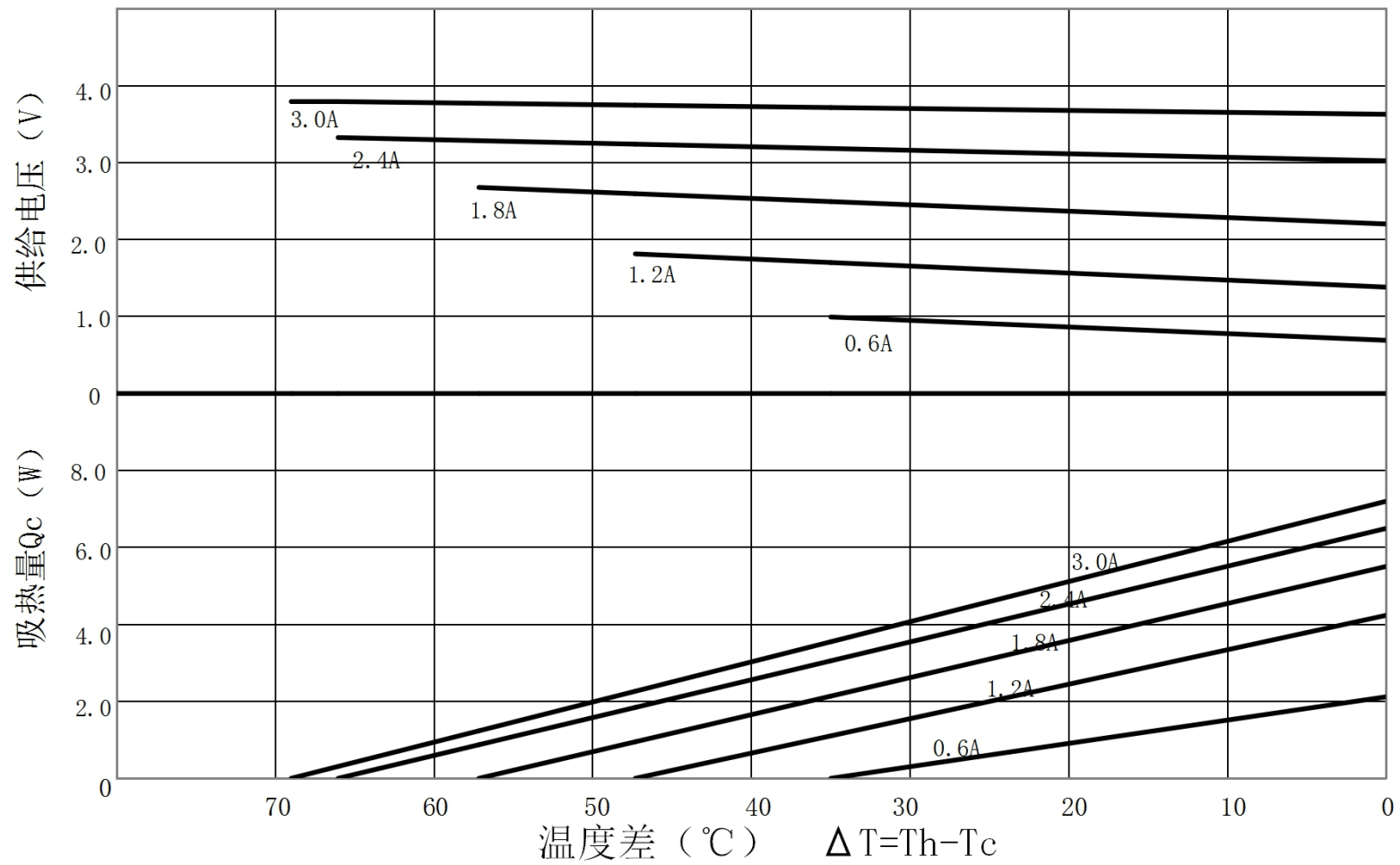
TEC1-B3103NC特性图 (Th=27°C)
