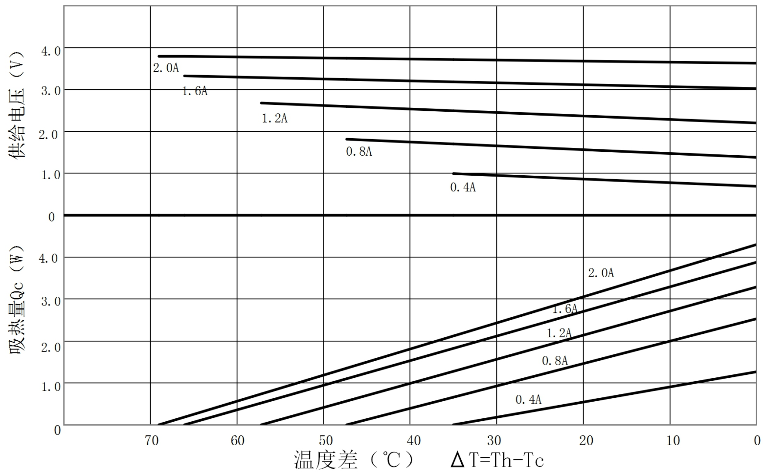
TEC1-B3102NC特性图 (Th=27°C)
