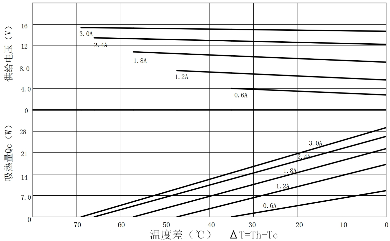
TEC1-B12703AC特性图 (Th=27°C)
