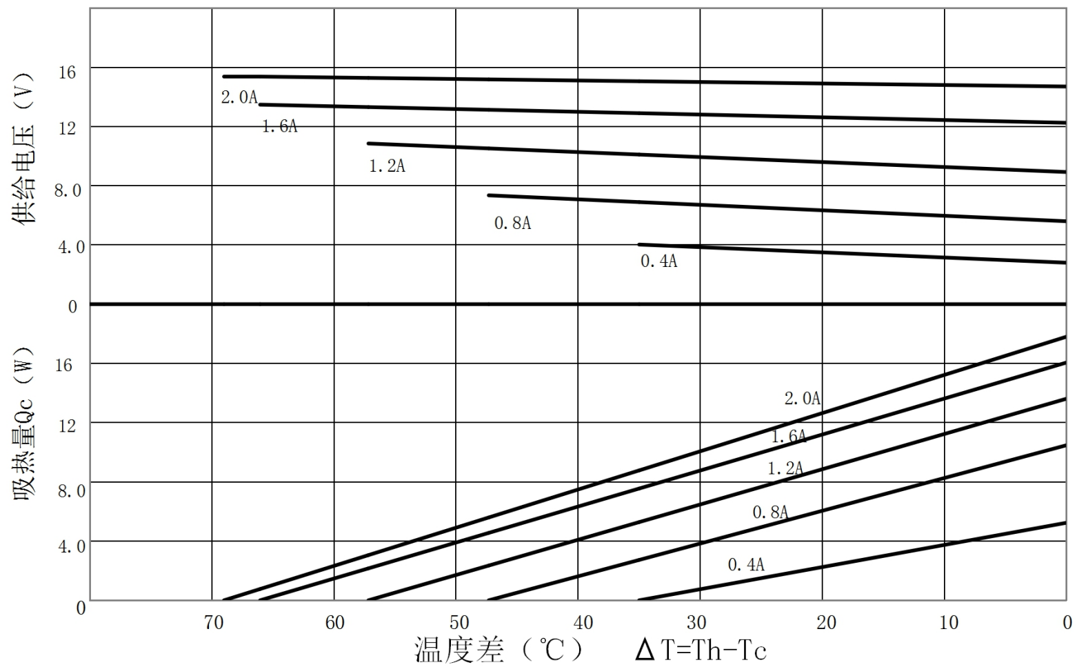
TEC1-B12702AC特性图 (Th=27°C)
