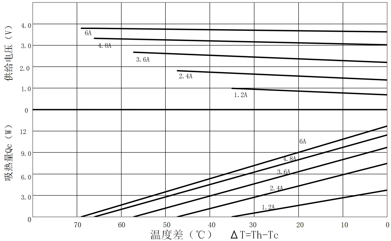
TEC1-B3106NC特性图 (Th=27°C)
