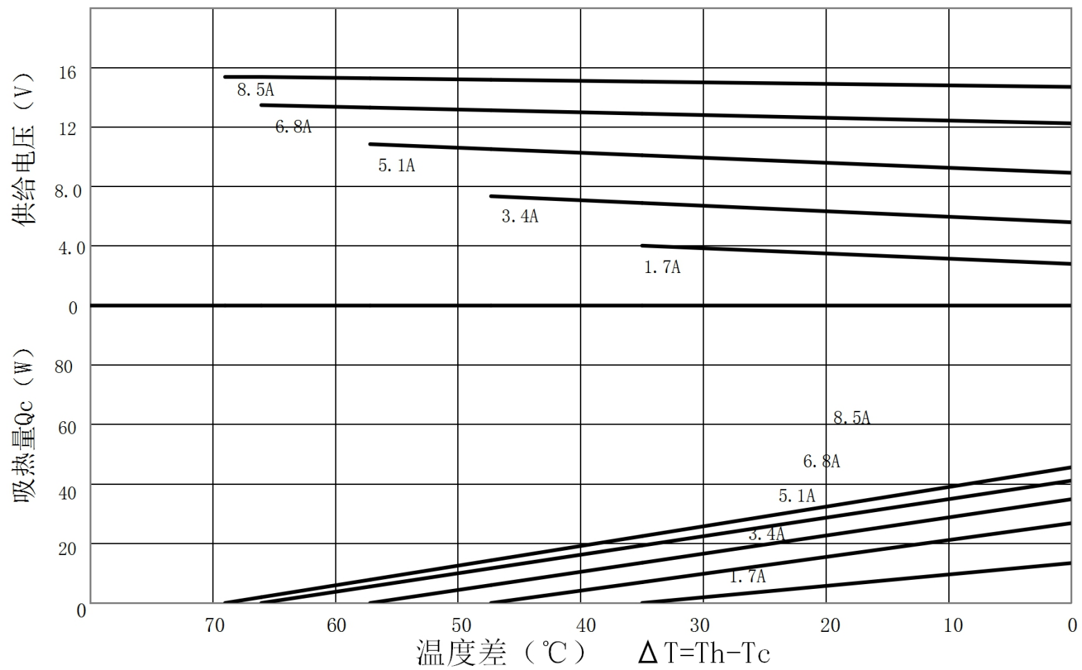
TEC1-B12708AC特性图 (Th=27°C)
