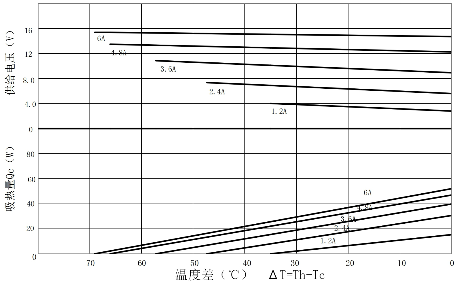
TEC1-B12706AC特性图 (Th=27°C)
