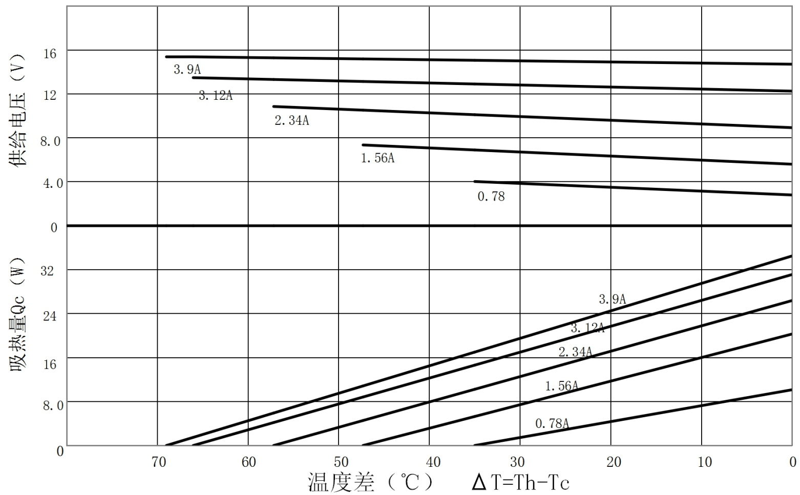
TEC1-B12704AC特性图 (Th=27°C)
