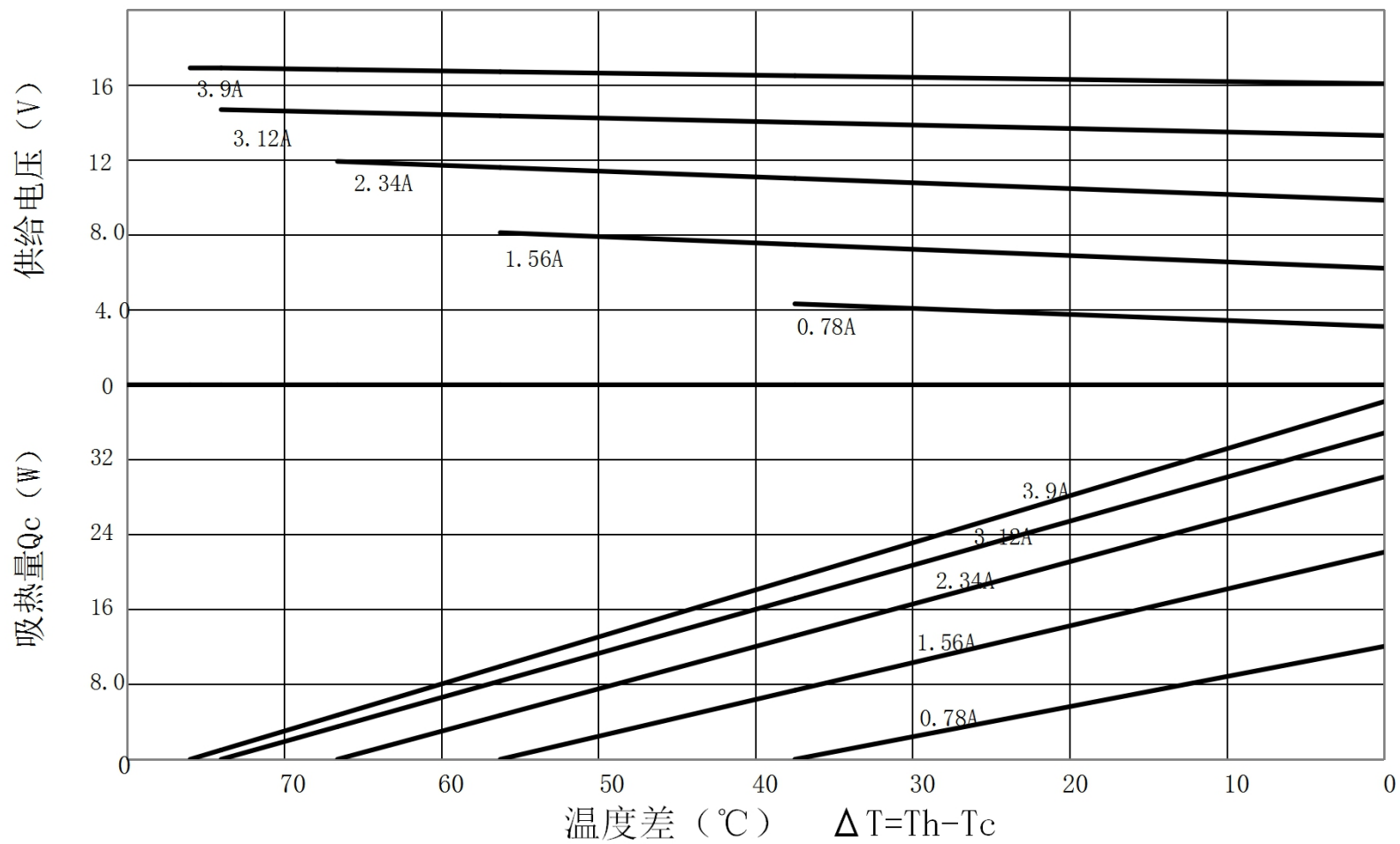
TEC1-B12704AC特性图 (Th=50°C)
